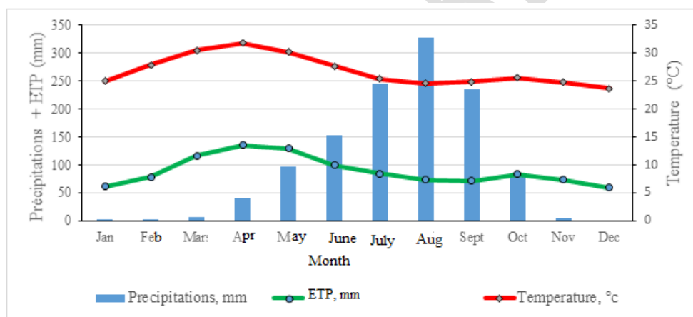
Figure 6. Umbro-thermal diagram for the study area (1981-2020)
