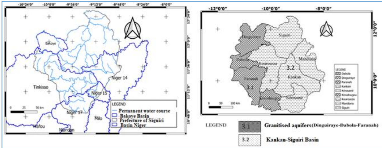
Figure 2: Sub-catchment areas of the River Niger in the Siguiri prefecture
