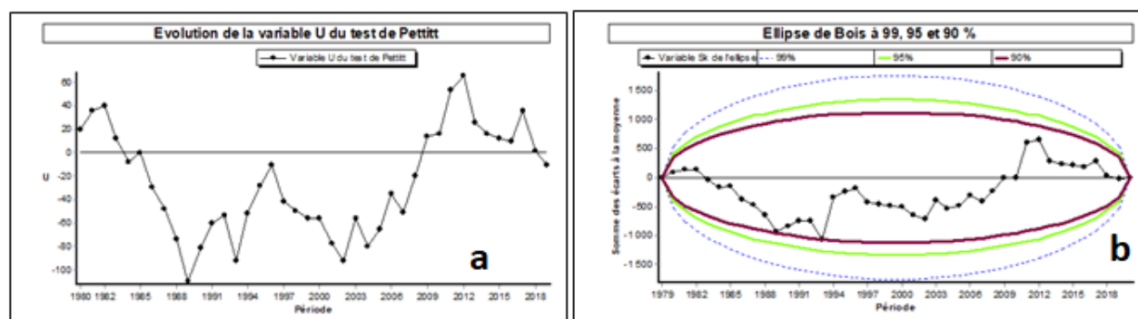
Figure 5. Pettitt statistical test (Figure 5a) and Bois Ellipse (Figure 5b) on annual rainfall
