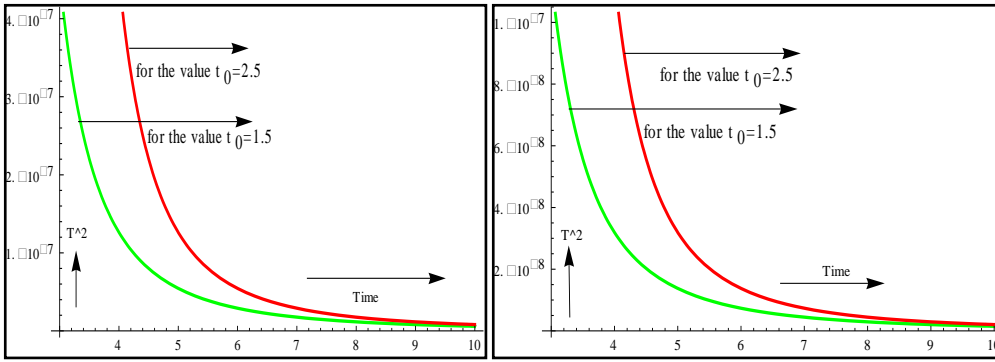
Figure-(2a): Sketch of equation(33)
