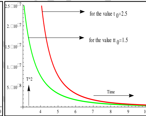
Figure-(4b):Sketch of equation(33)
