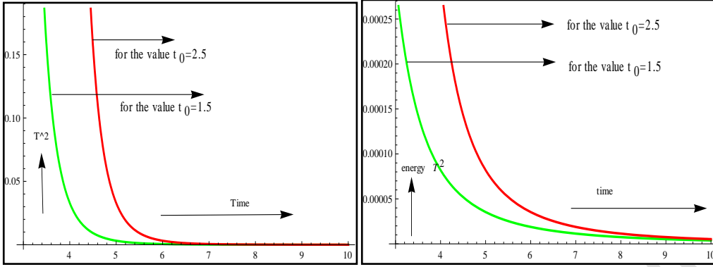
Fig (5a): Energy curves of equation. (33) Fig (5b): Energy curves of equation. (34)
