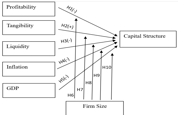
Figure 1. Research Framework
