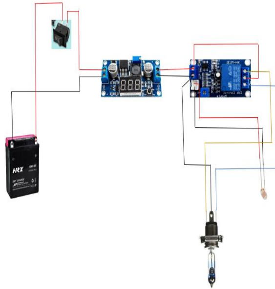
Figure 11. Schematic Diagram
