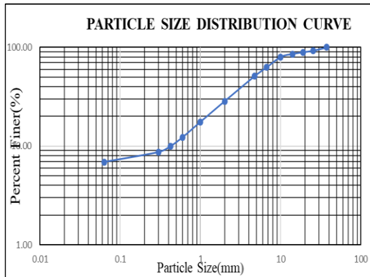
Figure-3: Particle Size Distribution of the Laterite
