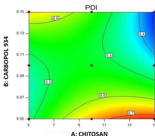
Figure. 04: The PDI is shown on the Surface plot, which demonstrates the impact of Chitosan and Carbopol 934 Concentration
