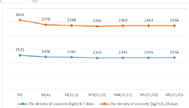
Figure 19: Density of 7 and 28 days of concrete
