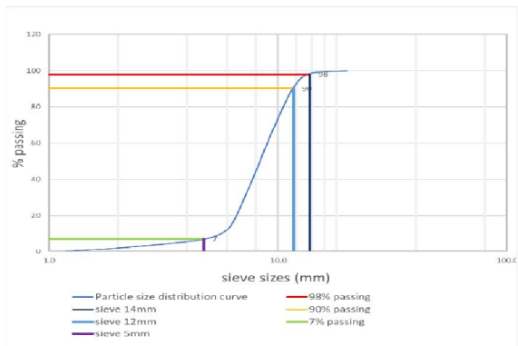
Fig. 15: Particles size distribution of PKS.
