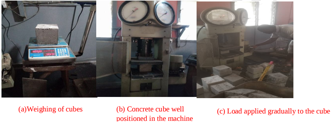
Fig. 12: Testing of cubes.
