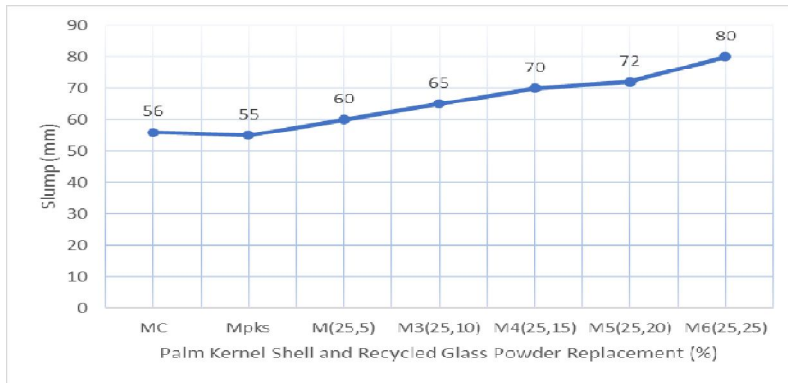
Fig. 17: Effect of Replacement of 25% PKS and RGP on Workability of Concrete.
