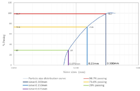
Fig. 13: Particle size distribution of RGP
