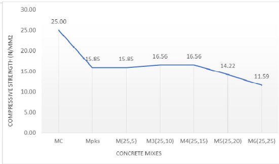
Fig. 21: 28 th day compressive concrete strength of various RGP with 25% PKS replacement to granitic coarse aggregate.
