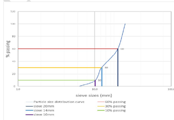
Fig. 14: Particle size distribution of coarse aggregate.
