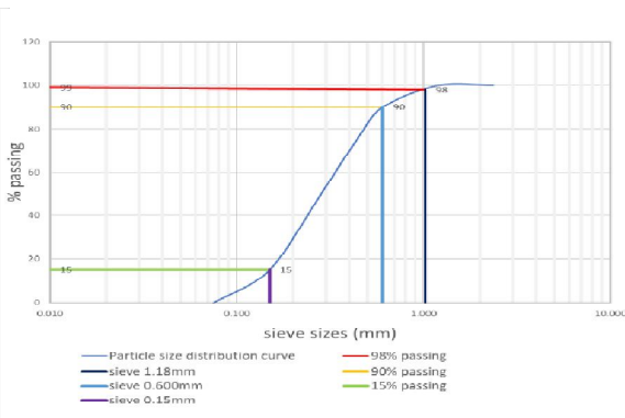
Fig. 16: Particles size distribution of fine aggregate
