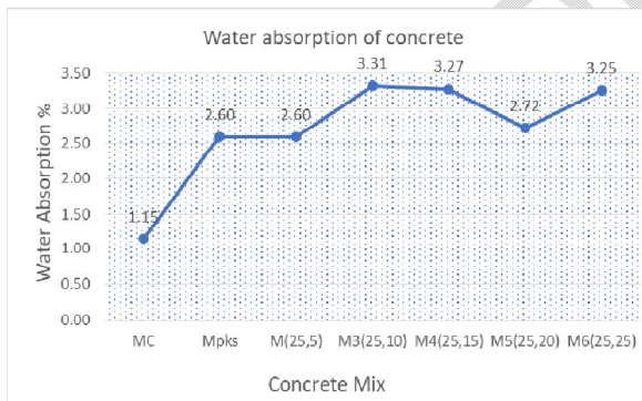
Fig. 18: Water Absorption of concrete
