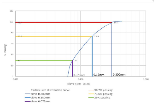
Fig. 13: Particle size distribution of RGP
