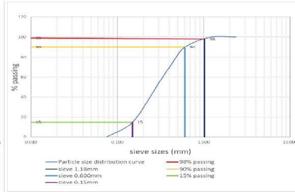
Fig. 16: Particles size distribution of fine aggregate
