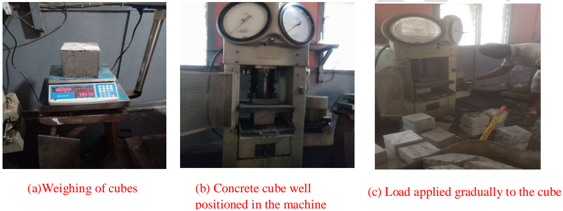
Fig. 12: Testing of cubes.
