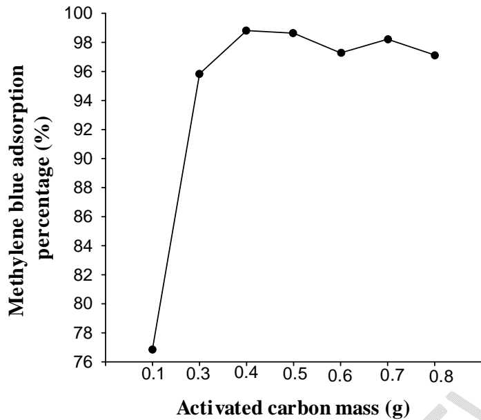
Fig. 4 Effect of activated carbon mass on methylene blue adsorption
