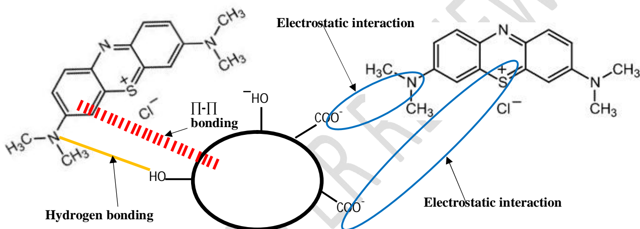
Fig. 8. Possible interaction and mechanism of methylene blue dye adsorption
