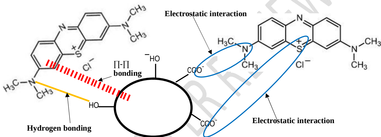
Fig. 8. Possible interaction and mechanism of methylene blue dye adsorption
