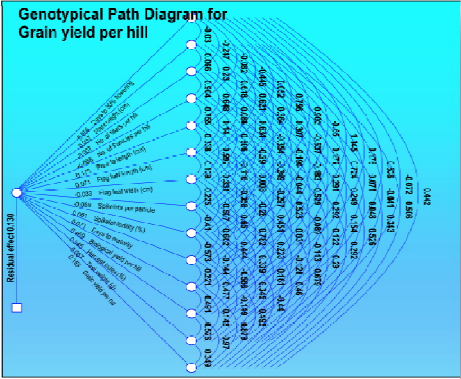
Fig. 1. Genotypic Path Coefficient
