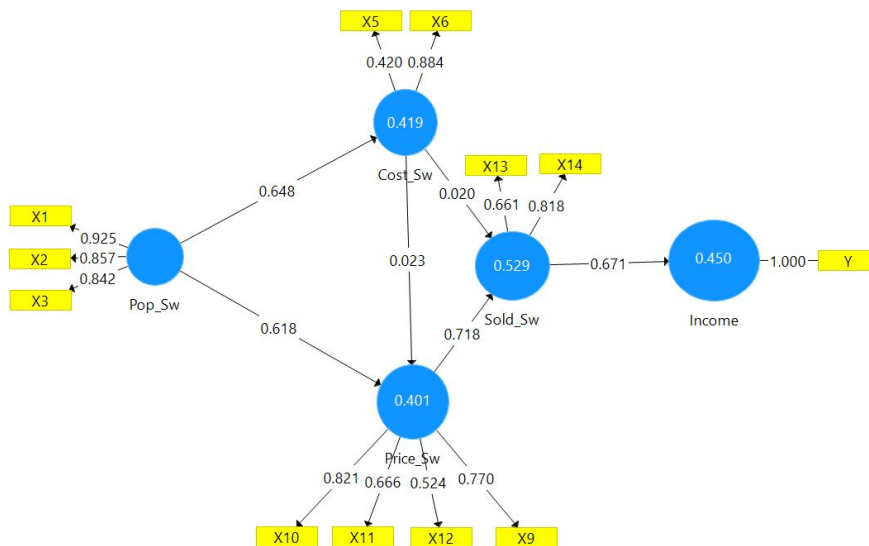
Figure 2. Results of the first analysis for checking loading factor values. X1:Population piglet, X2:Population weaners, X3:Population adults, X5: Cost medicine, X6:Cost feed, X9:Price weaners, X10: Price adult, X11: Total price, X12: Cost total, X13: Sold piglet, X14: Sold weaners, Y:Income
