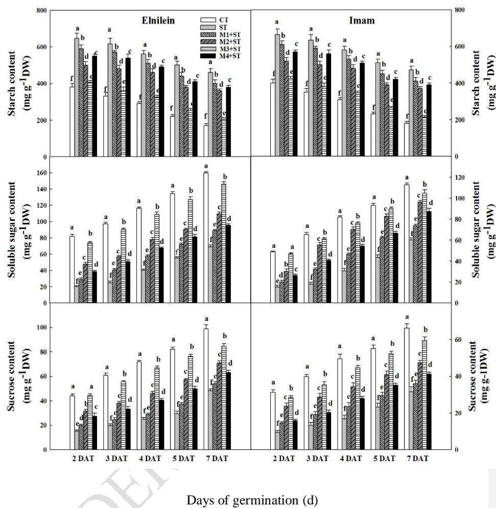
Fig. 1 Effect of melatonin priming on changes in contents of starch, soluble sugar, and sucrose in wheat seeds during 7 days germination under salt stress. Data are means \pm SD ( n=3 ). Different small letters at each day indicate significant difference between treatments at P < 0.05 .
