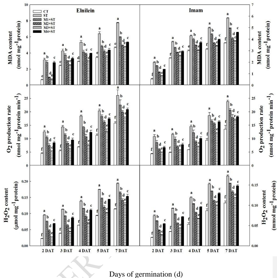
Fig.3 Effect of melatonin priming on changes in contents of malondialdehyde (MDA), hydrogen peroxide ( H_2O_2 ), and O_2 production rate in wheat seeds during 7 days germination under salt stress. Data are means \pm SD (n=3). Different small letters at each day indicate significant difference between treatments at P < 0.05
