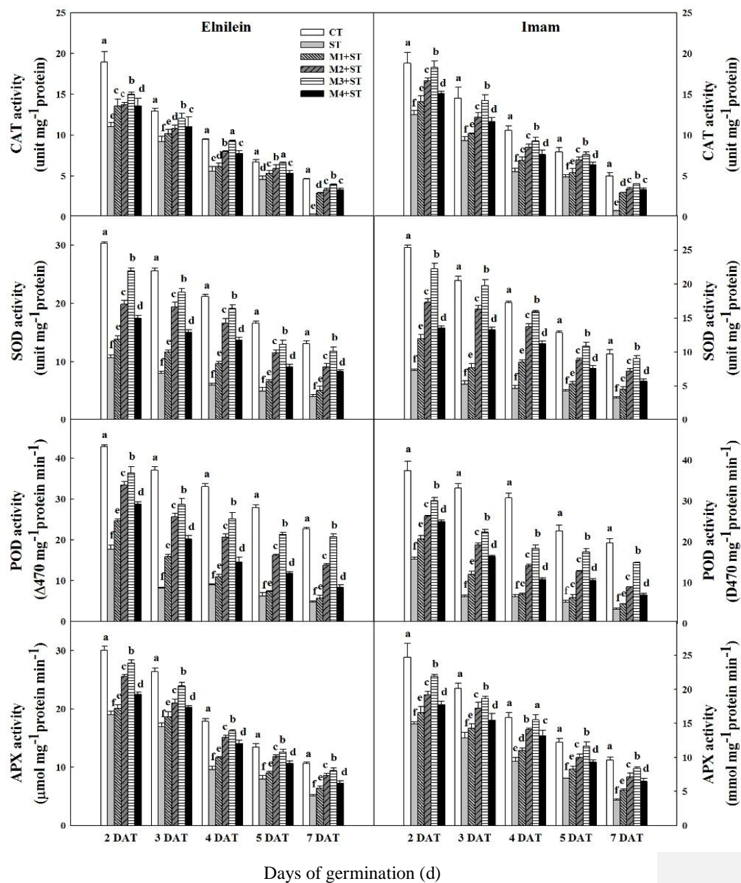
Fig. 4 Effect of melatonin priming on changes in activities of superoxide dismutase (SOD), catalase (CAT), peroxidase (POD), and ascorbate peroxidase (APX) in wheat seeds during 7 days germination under salt stress. Data are means \pm SD (n=3). Different small letters at each day indicate significant difference between treatments at P < 0.05
