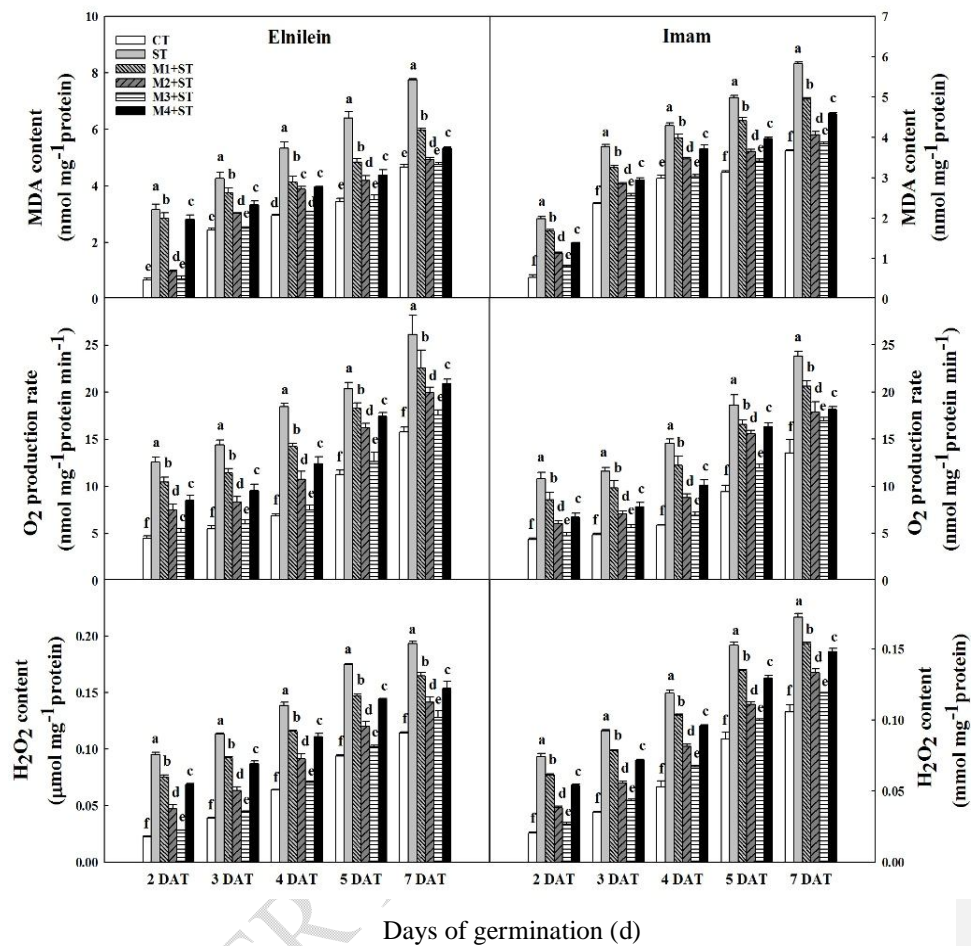
Fig.3 Effect of melatonin priming on changes in contents of malondialdehyde (MDA), hydrogen peroxide ( H_2O_2 ), and O_2 production rate in wheat seeds during 7 days germination under salt stress. Data are means \pm SD (n=3). Different small letters at each day indicate significant difference between treatments at P < 0.05
