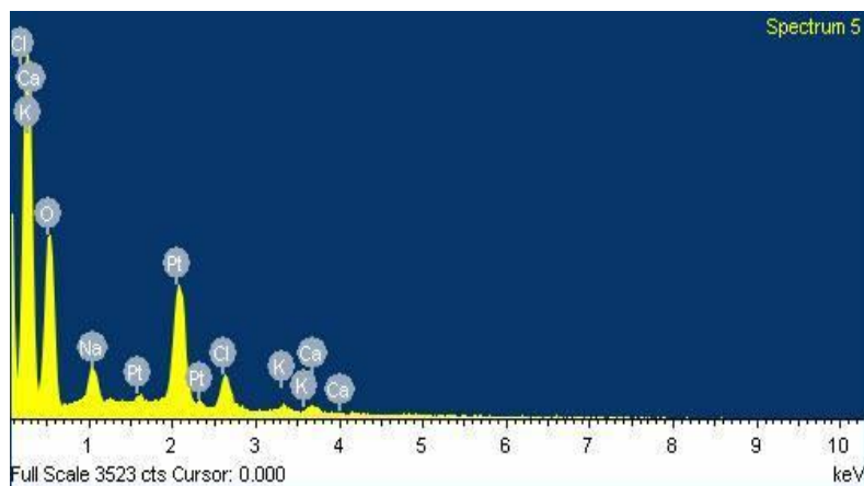
Fig 2: EDX of Sweet Lime Peel Powder (SLPP)
