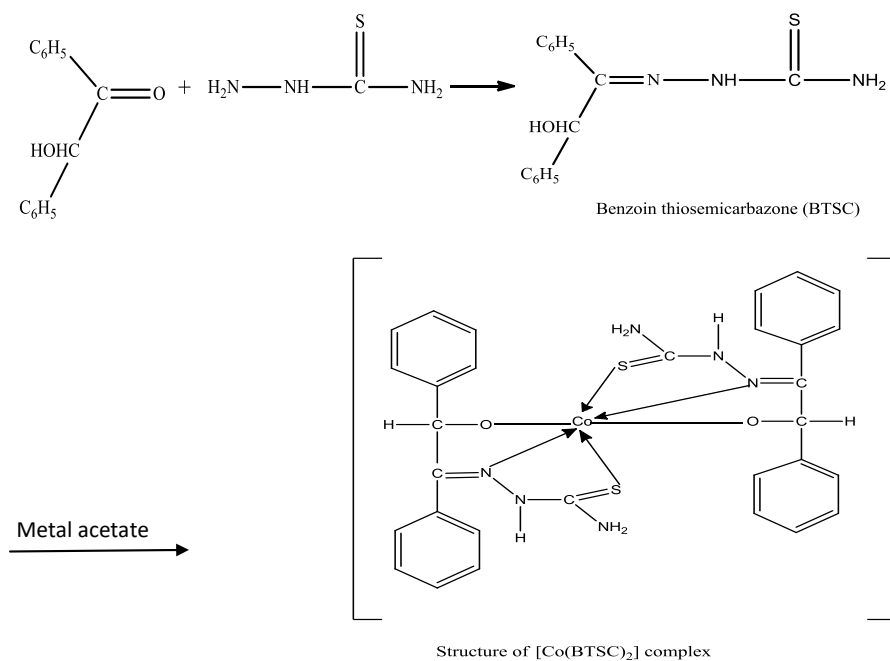
Figure- 1: Synthesis of Co(II)-benzoin thiosemicarbazone complex
